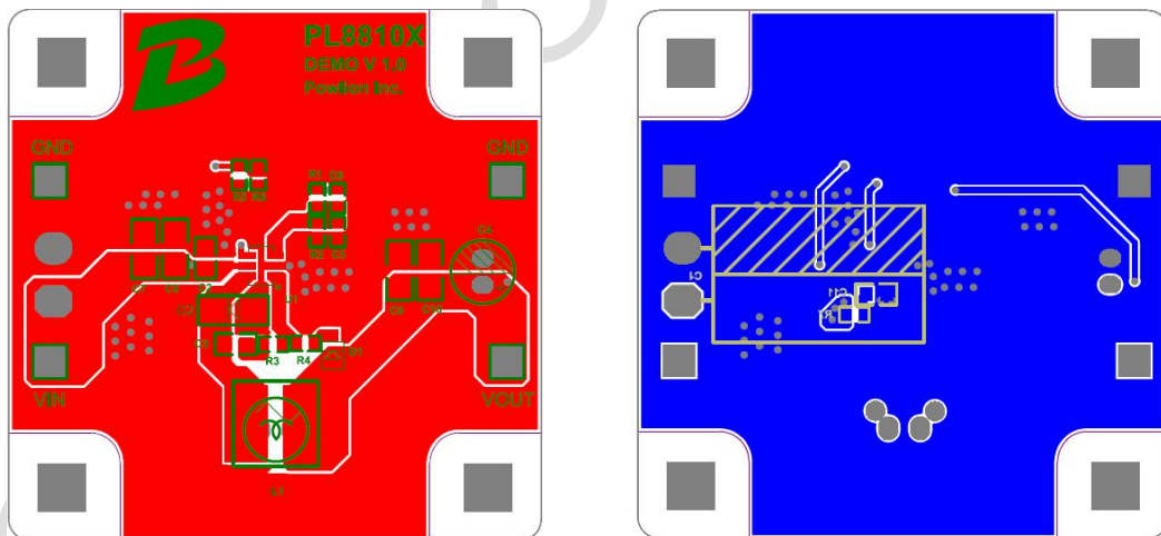
Fig 25 PCB Layout
