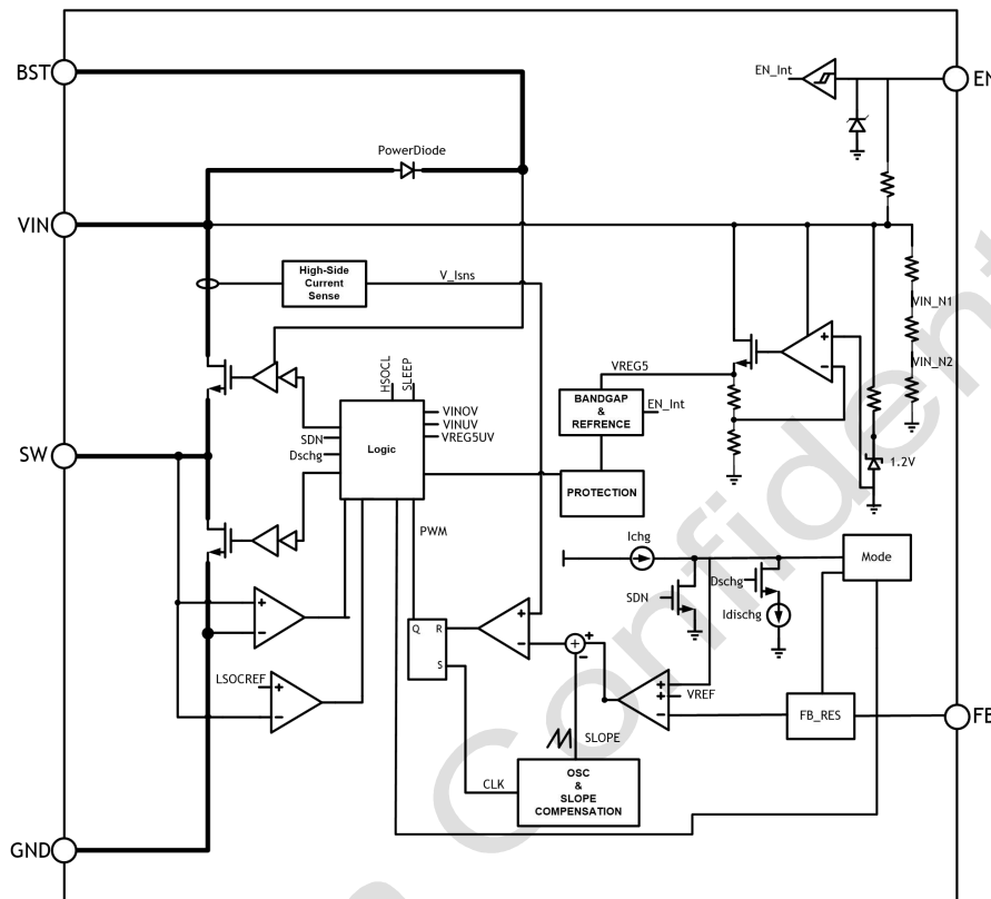
Fig.22 PL88104 Diagram
