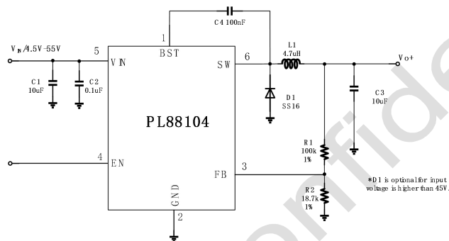
Fig 24 Schematic
